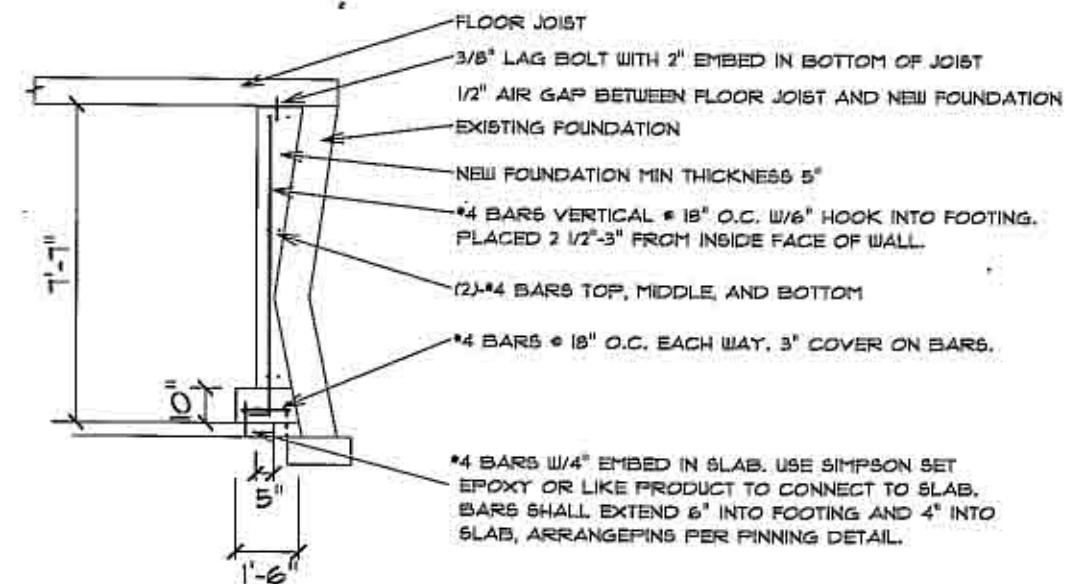
REPAIR FOR WEST BASEMENT FOUNDATION WALL
