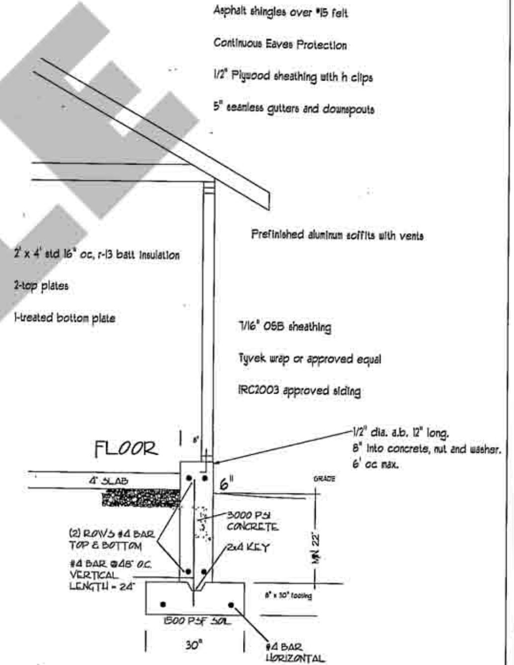
WALL DETAIL AND FROST WALL DETAIL
