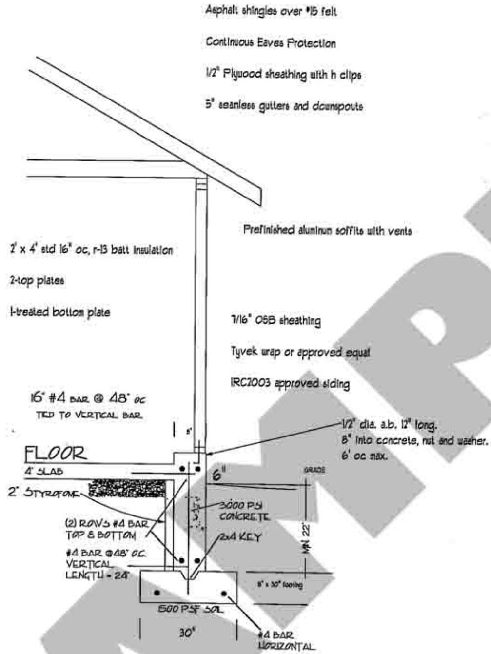
Alternate "One Pour" Slab and stem wall
